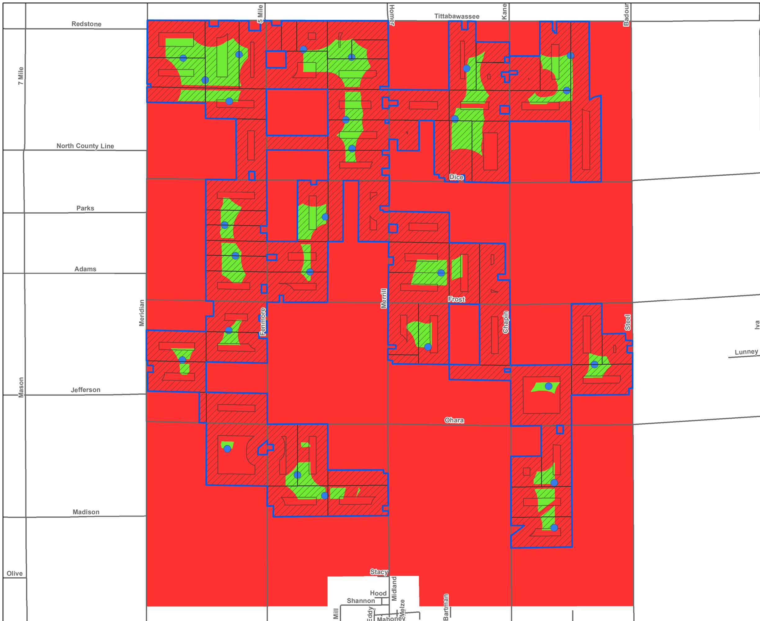
Turbine Layout r21
